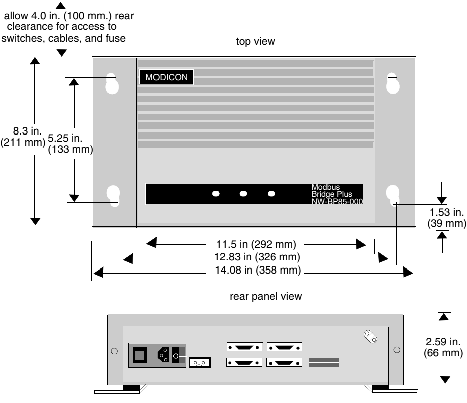
BP85 bridge plus dimensions (panel/shelf models)
