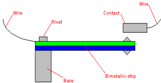
Figure 12 Bimetallic Thermostat
