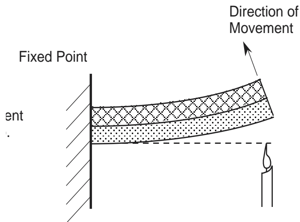
Figure 11 Bimetallic Strip Bent after Heat is Applied
