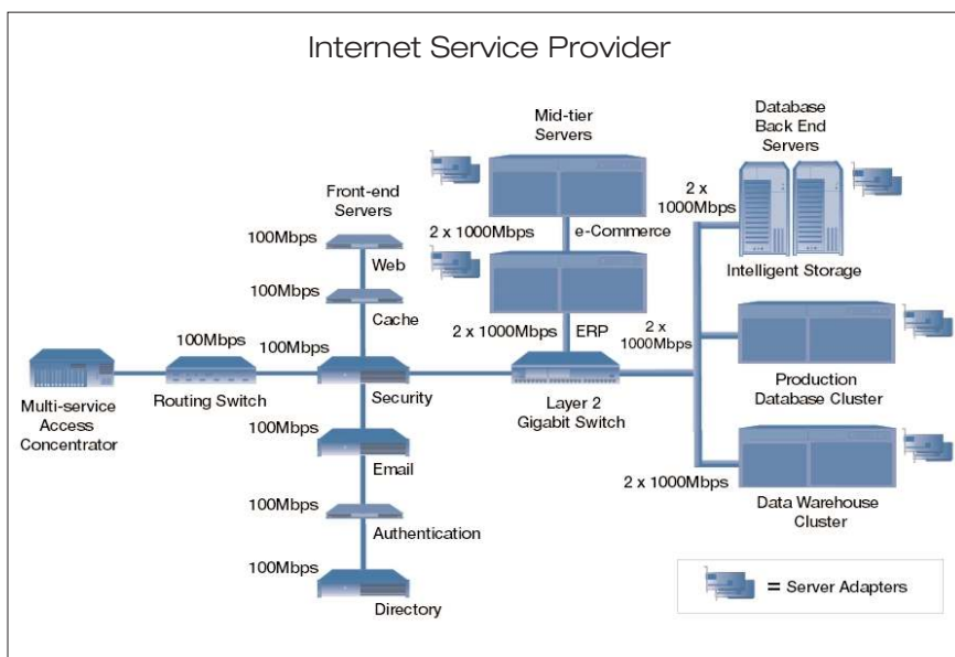
Figure 8, Deployment at an ISP.
