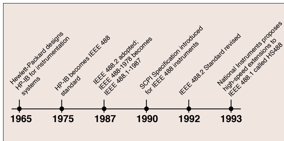
Figure 1. GPIB History
