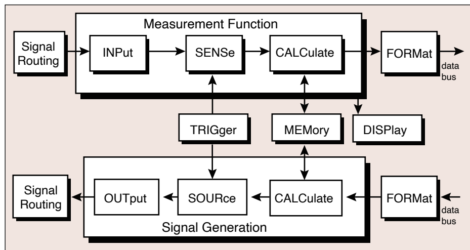
Figure 10. The SCPI Instrument Model
