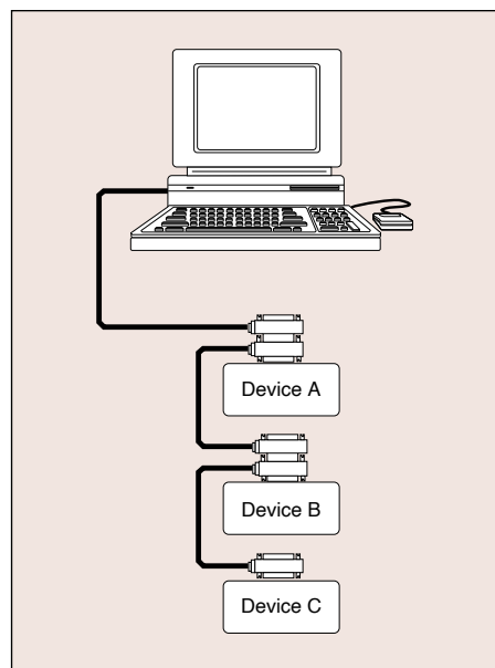
Figure 4. Linear Configuration
