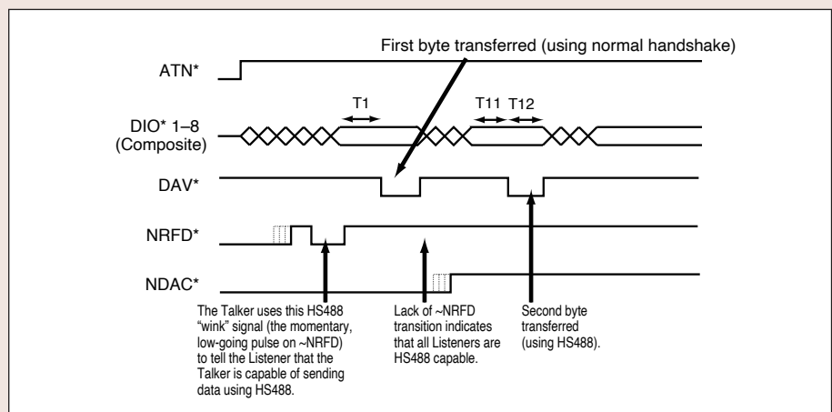
Figure 8. HS488 Handshake
